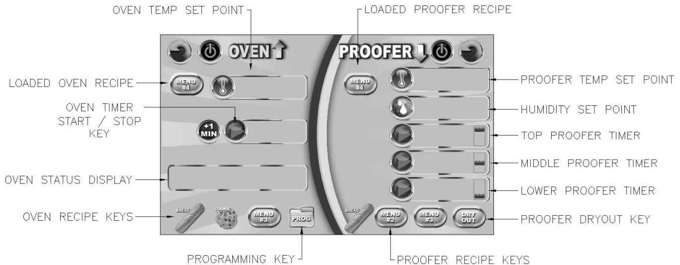
Fig. #4 –Oven & Proofer Controls
